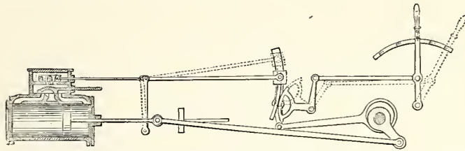
Fig. 11.—VARIABLE CUT-OFF ADJUSTMENT.
